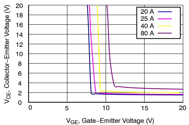
Figure 6. Saturation Voltage vs. V_{GS} (175°C)
